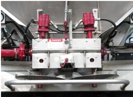
Top mounted hydraulic motors with 24" spinner plates and stainless steel back plate and bumper
